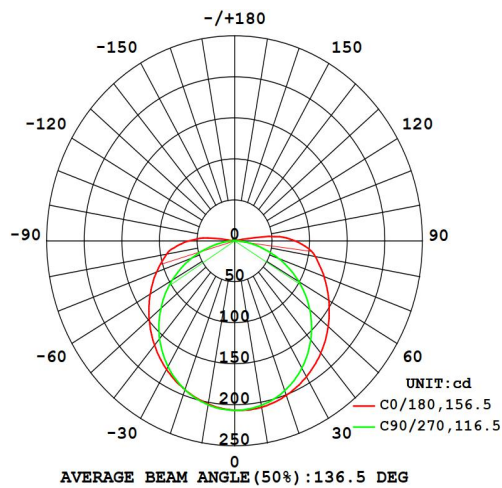
Photometric of 1M (6500K) strip
