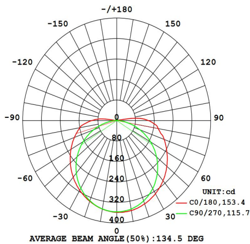
Photometric of 1M (2700K+6500K) strip
