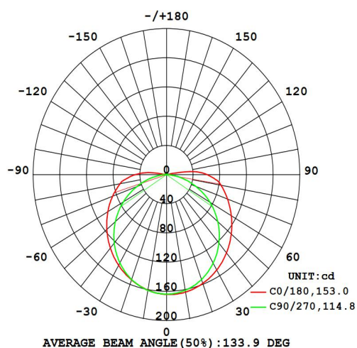
Photometric of 1M (2700K) strip
